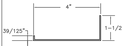
FLANGE FRAME HEAD AND SILL
