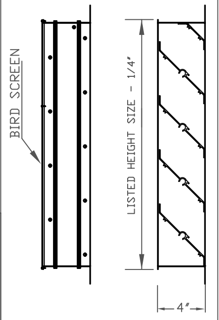
FLANGE FRAME HEAD AND SILL
