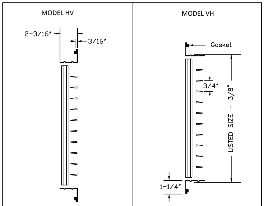
STANDARD FASTENING DETAIL
